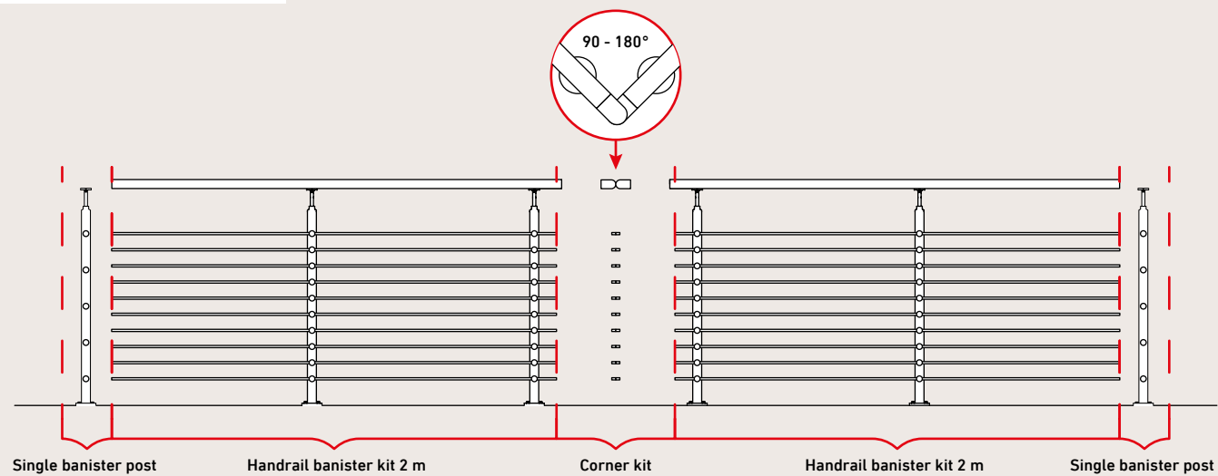
EXAMPLE OF CORNER KIT
